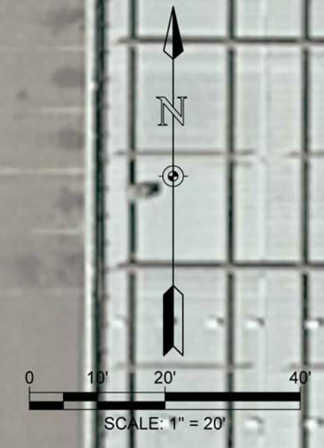
DELL RANGE BLVD. AND WALMART ACCESS INTERSECTION IMPROVEMENTS
