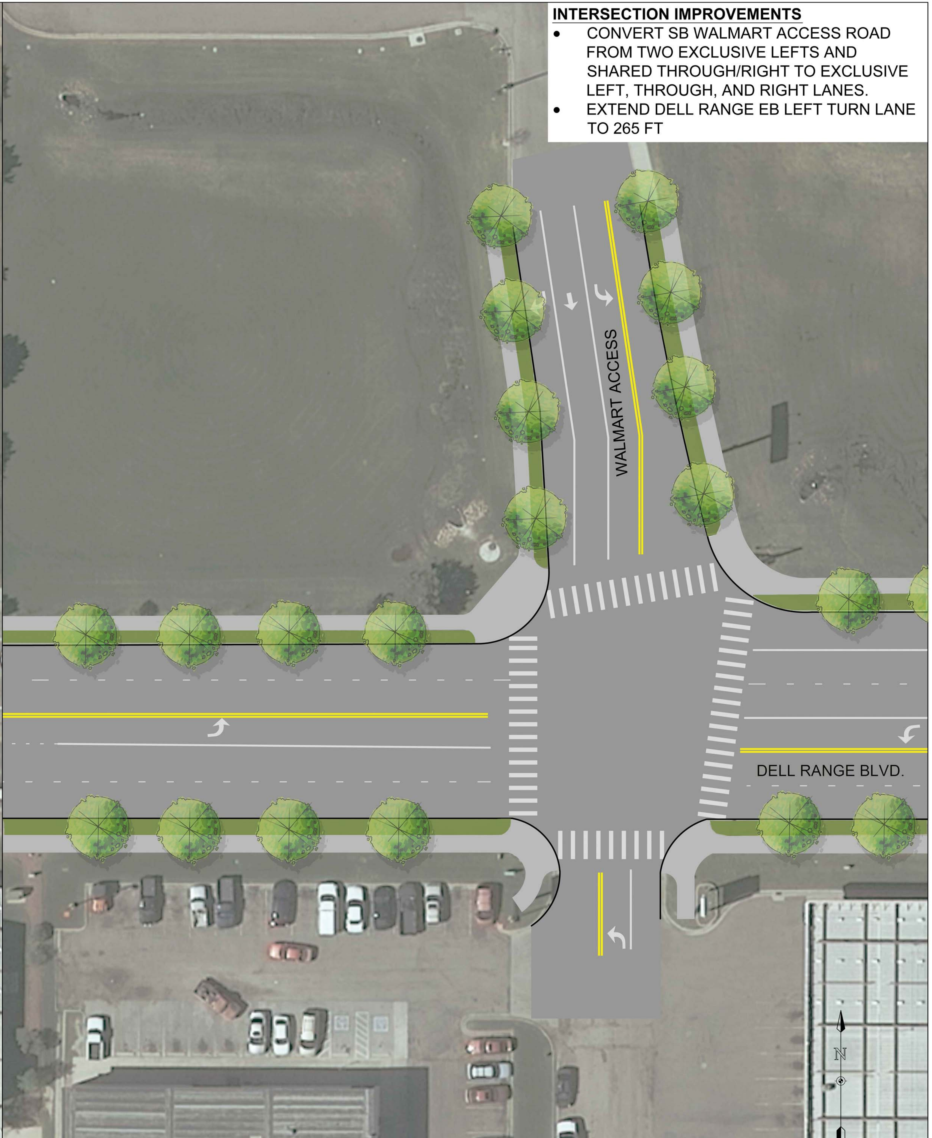
DELL RANGE BLVD. AND WALMART ACCESS INTERSECTION IMPROVEMENTS
