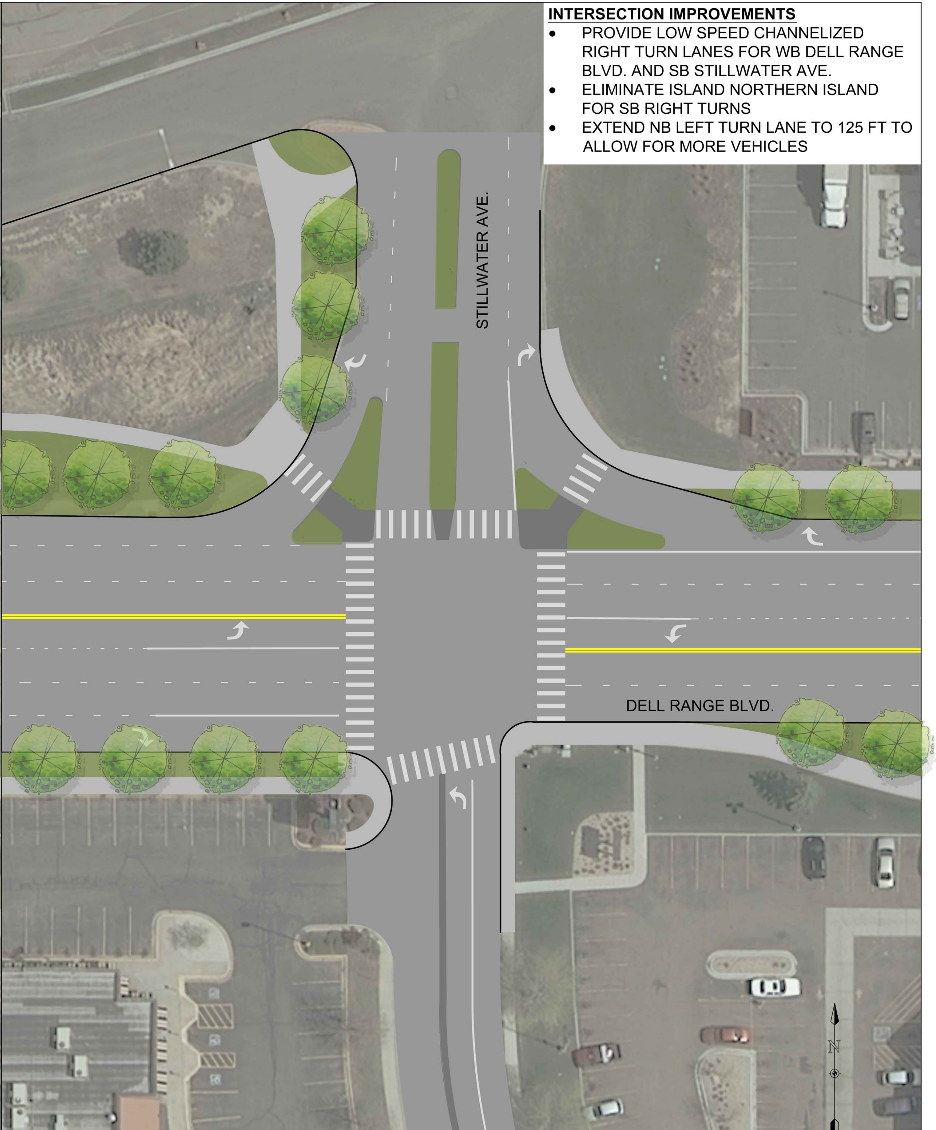
DELL RANGE BLVD. AND STILLWATER AVE. INTERSECTION IMPROVEMENTS
