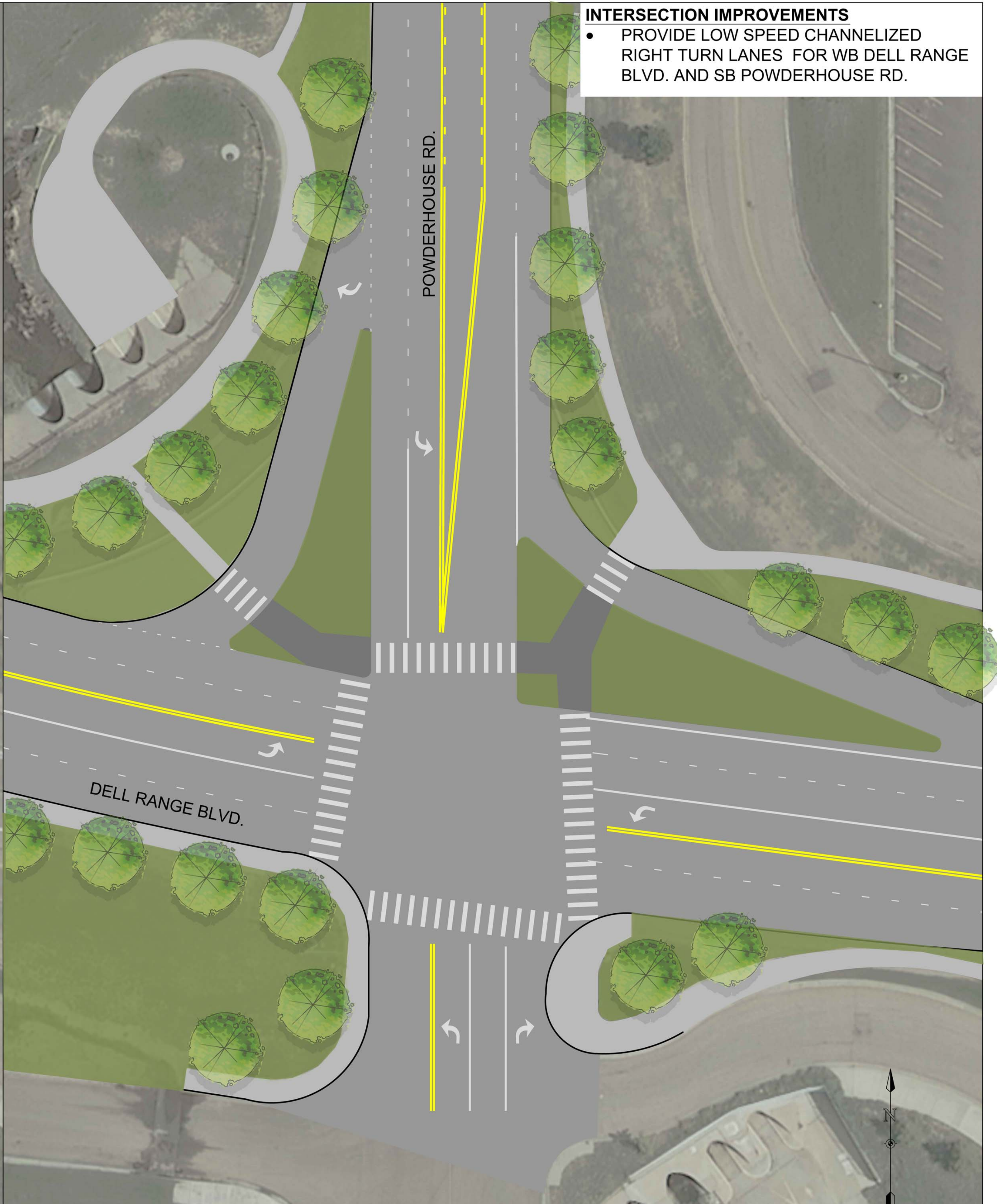
DELL RANGE BLVD. AND POWDERHOUSE RD. INTERSECTION IMPROVEMENTS
