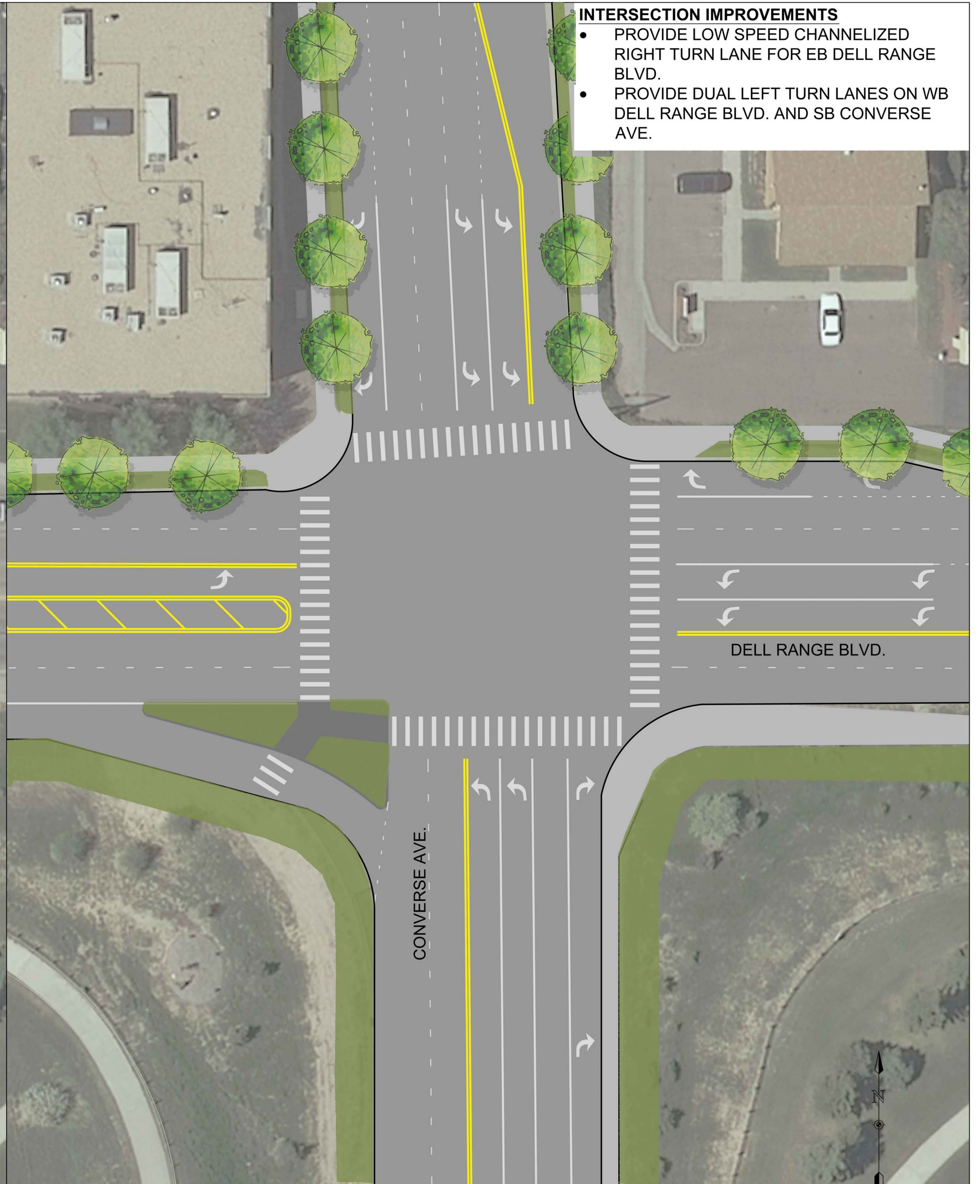
DELL RANGE BLVD. AND CONVERSE AVE. INTERSECTION IMPROVEMENTS
