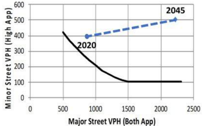
Figure 7: Year 2045 Peak Hour Traffic Signal Warrant Enhanced 3-Lane Roadway Alternative Mason Way
