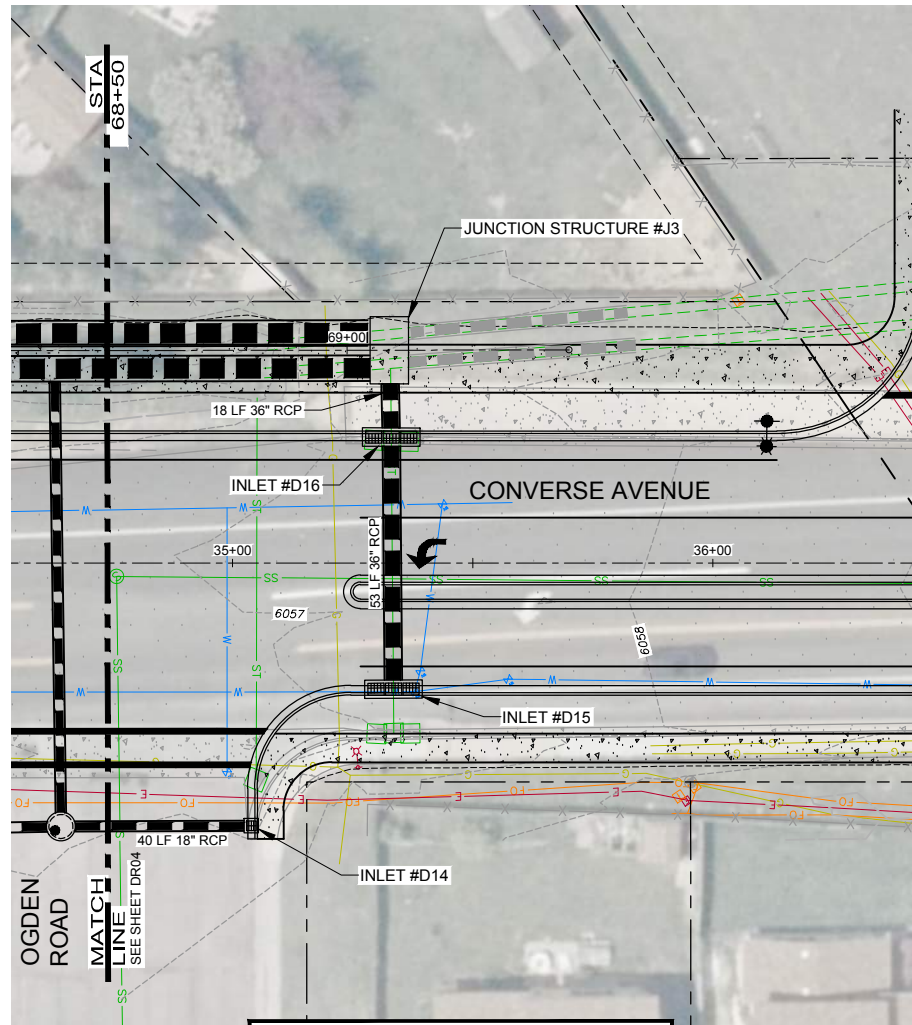
STORM DRAINAGE PLAN AND PROFILE
