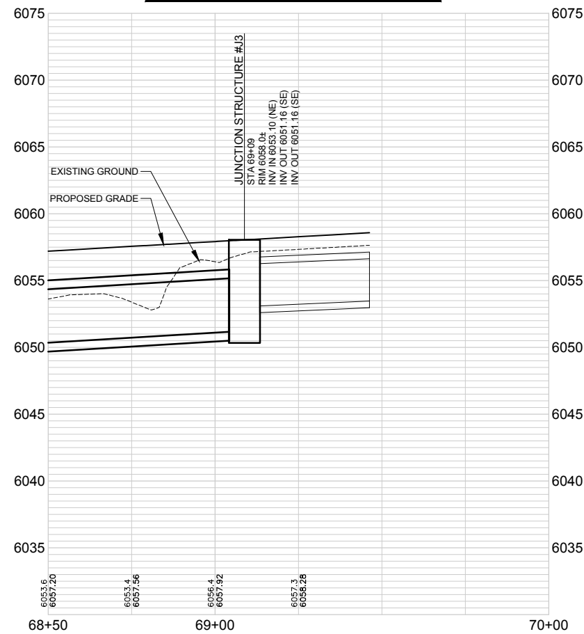
STORM DRAINAGE PLAN AND PROFILE
