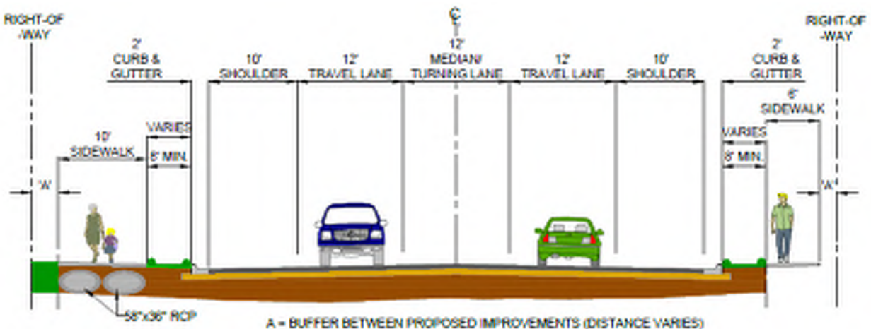
Figure 4-1 - Typical Section
